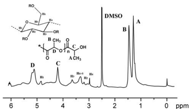
Figure 2. ^1\text{H} -NMR spectrum of cellulose-g-PLLA ( \text{DP}_{\text{PLLA}} = 3.15 ) in \text{DMSO}-d_6 .
