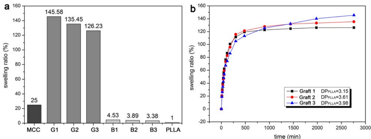
Figure 6. Degree of hydration of cellulose/PLLA blends and cellulose-g-PLLA. [Color figure can be viewed in the online issue, which is available at wileyonlinelibrary.com .]
